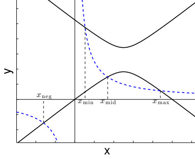
Figure 6: Critical points of \Phi_0(x, y) subject to the constraint xy = d .
