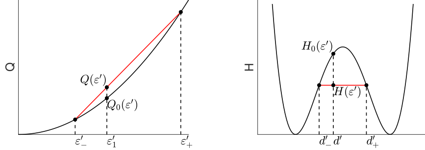
Figure 5: Geometric interpretation of functions Q(\boldsymbol{\varepsilon}') and H(\boldsymbol{\varepsilon}') .
