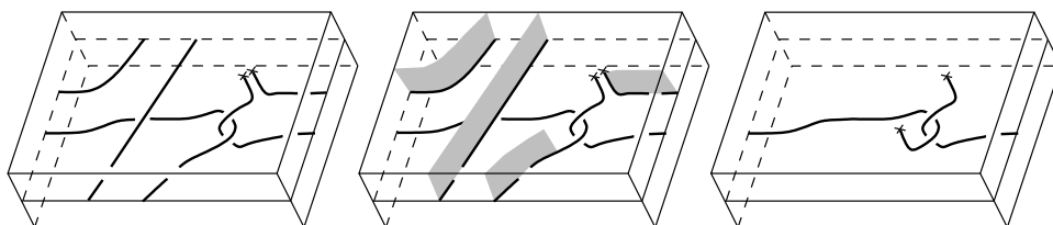
Figure 14: Manifolds homeomorphic to X \setminus \sigma_1
