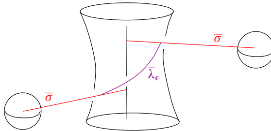
Figure 3: \bar{\sigma} is the geodesic in the homotopy class of the image of \sigma in the filled manifold X(\mu) . The curve \bar{\lambda}_\epsilon is the shortest curve along the \epsilon -Margulis tube between points where \bar{\sigma} meets the tube on its boundary. Picture in the universal cover.
